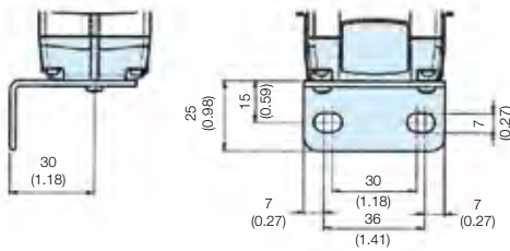
Foot Bracket
